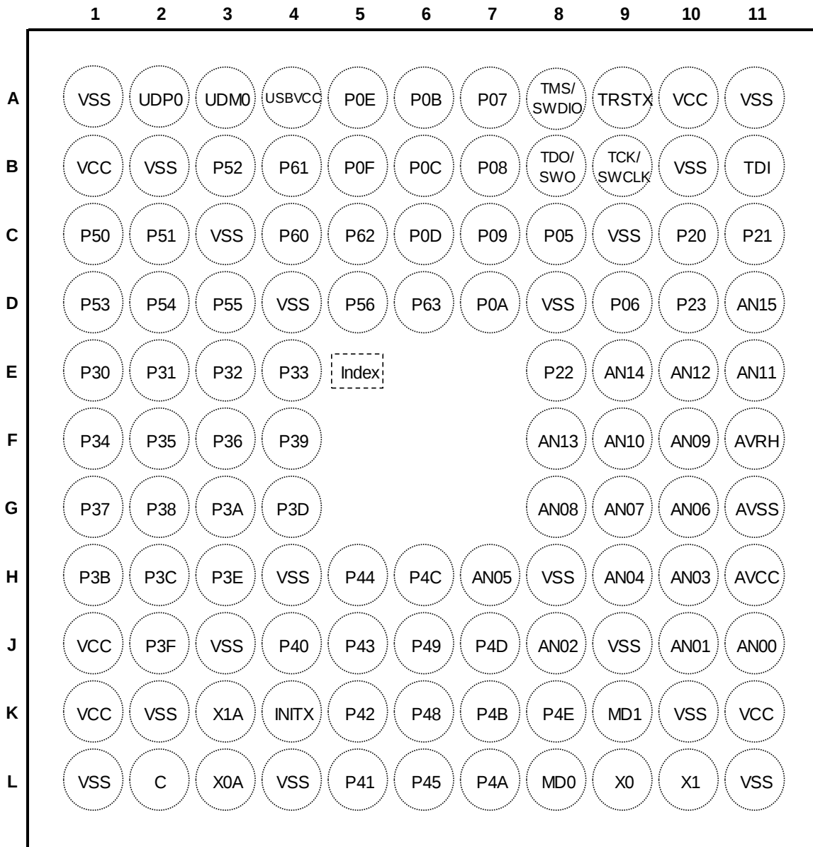
(TOP VIEW)
