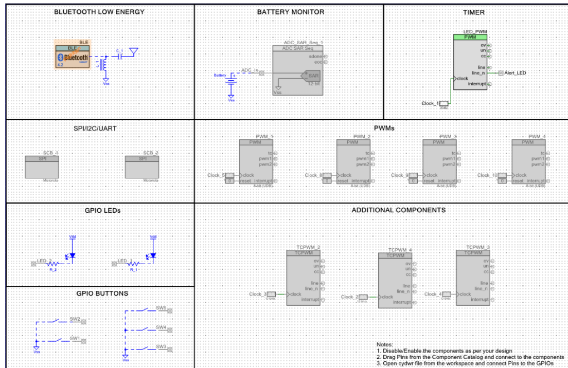
Figure 4-50. BLE_Dongle_Peripheral_IAS TopDesign
