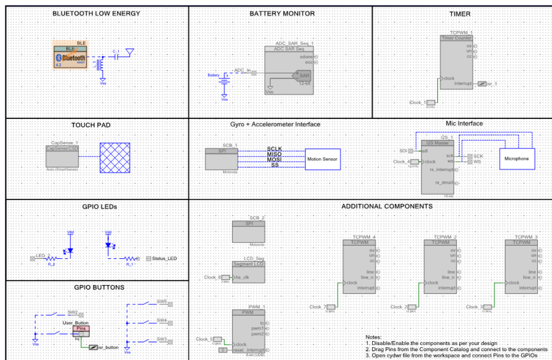
Figure 4-49. PRoC_BLE_Central_IAS TopDesign
