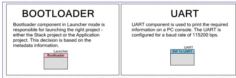
Figure 4-76. TopDesign for PSoC_4_BLE_OTLA_Launcher Project
