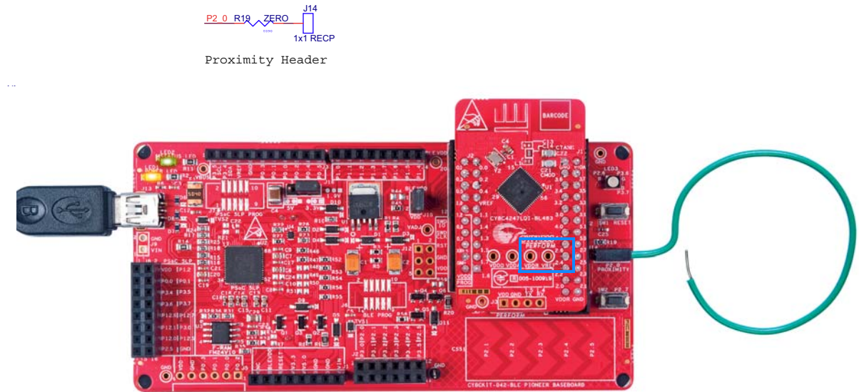
Figure 5-14. Schematics and Board Highlight of Proximity Header
