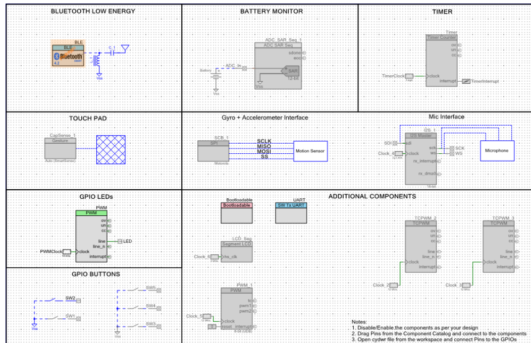
Figure 4-81. TopDesign for PProC BLE Original and New Application Projects
