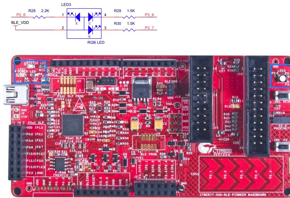
Figure 5-16. Schematics and Board Highlight of RGB LED
