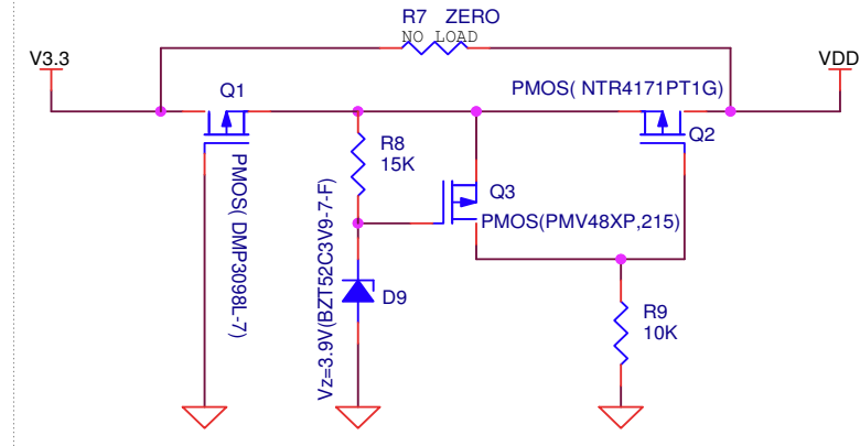
Figure 5-4. Schematics and Board Highlight of MOSFET Protection Circuit for 3.3-V Rail from J1.5
