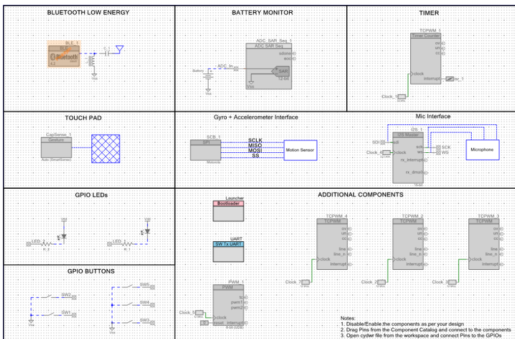
Figure 4-77. TopDesign for PSoC_BLE_OTLA_Launcher Project
