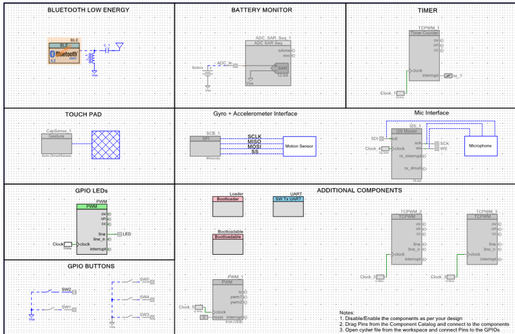
Figure 4-79. TopDesign for PSoC_4_BLE_OTA_Stack Project
