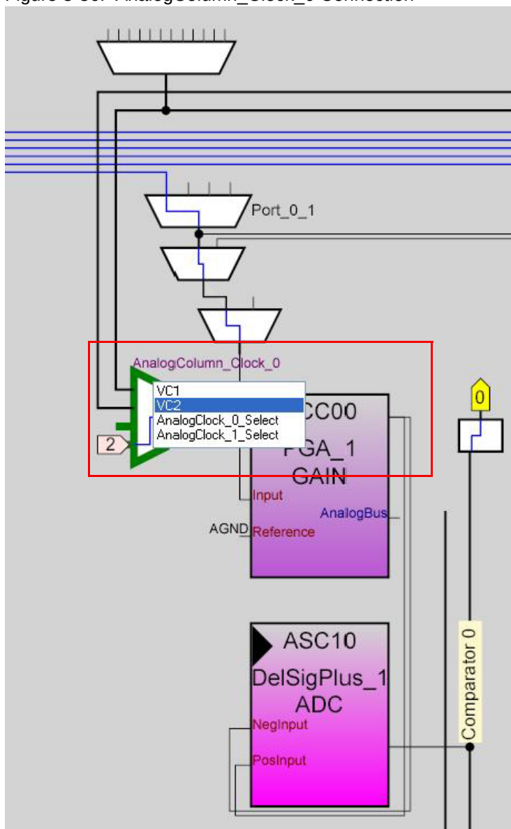
Figure 3-36. AnalogColumn_Clock_0 Connection
