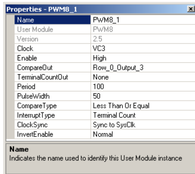
Figure 3-56. Properties Window
