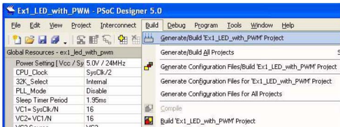
Figure 2-2. Build Project
