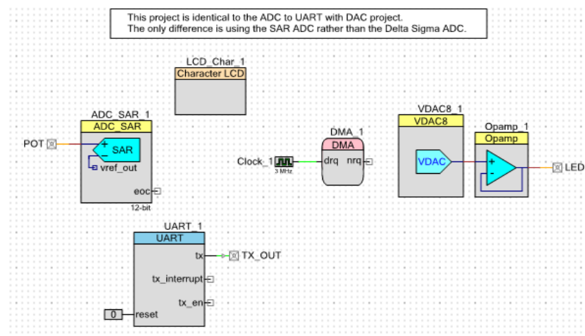
Figure 3-157. Connected Components
