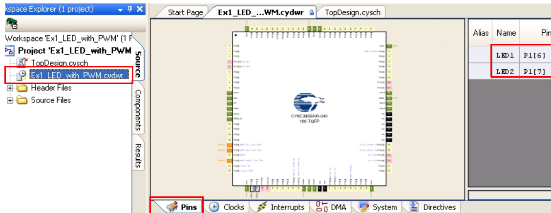
Figure 3-100. Pin Assignments
