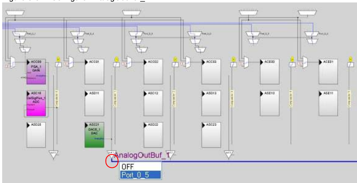
Figure 3-34. Configure AnalogOutBuf_1
