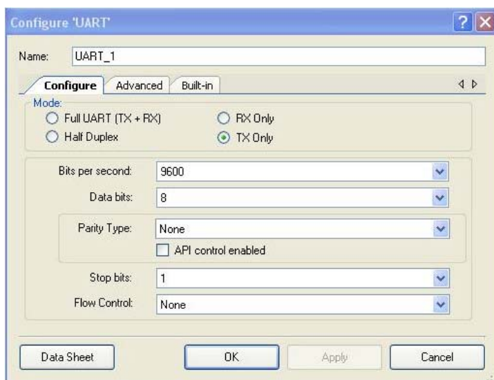
Figure 3-152. UART Component Configuration
