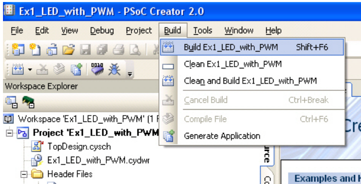
Figure 2-20. Build Window
