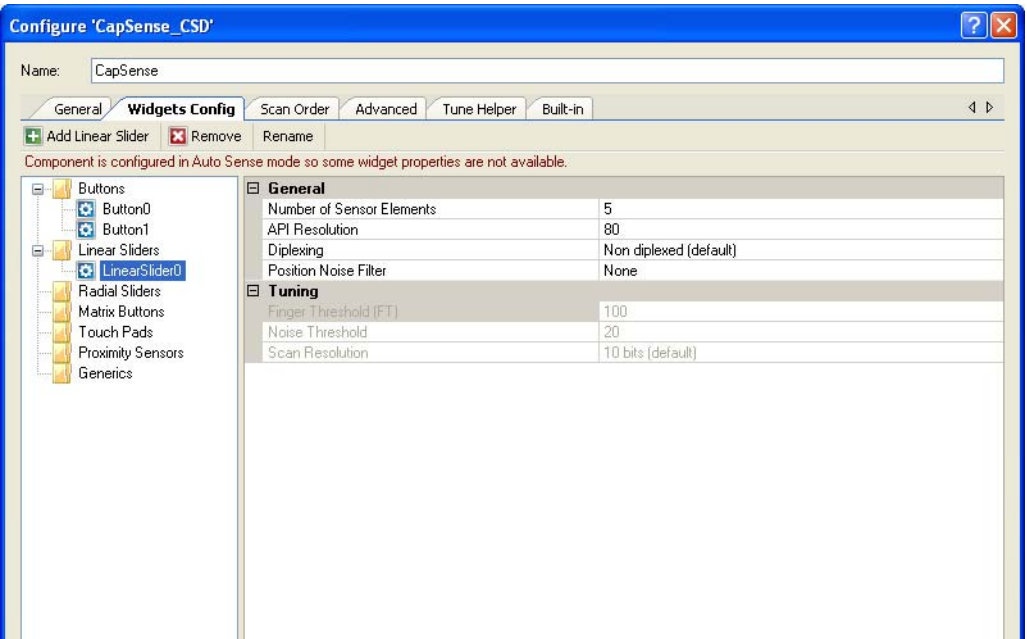
Figure 3-138. Slider Configuration
