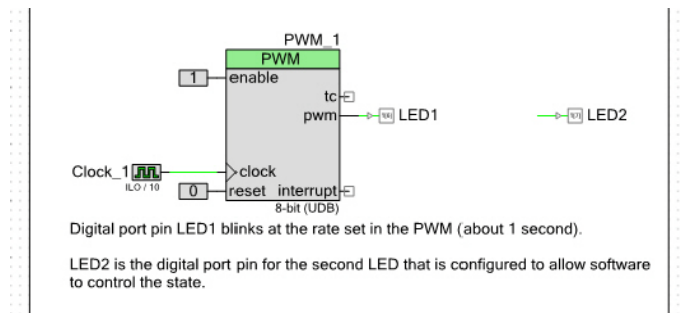
Figure 3-99. Connected Components
