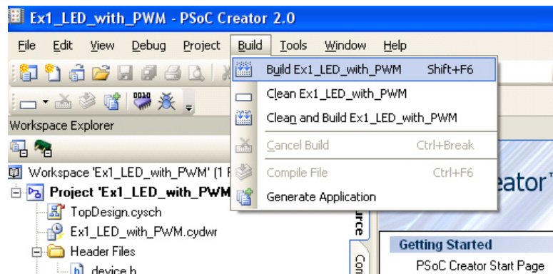
Figure 2-14. Build Window
