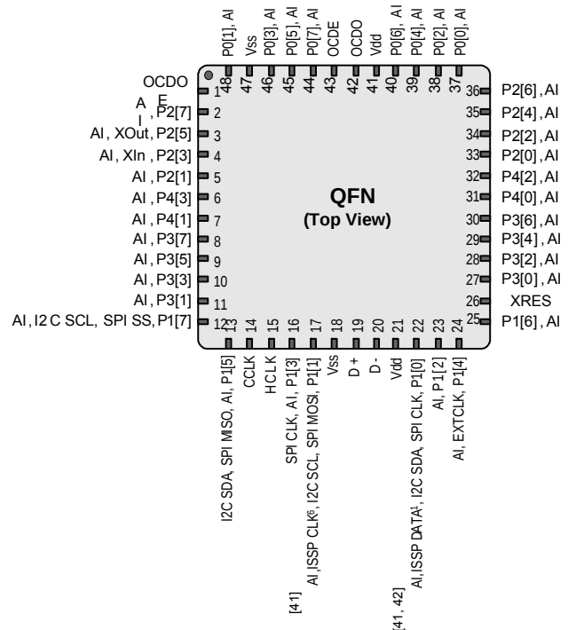
Figure 11. CY8C20066A
