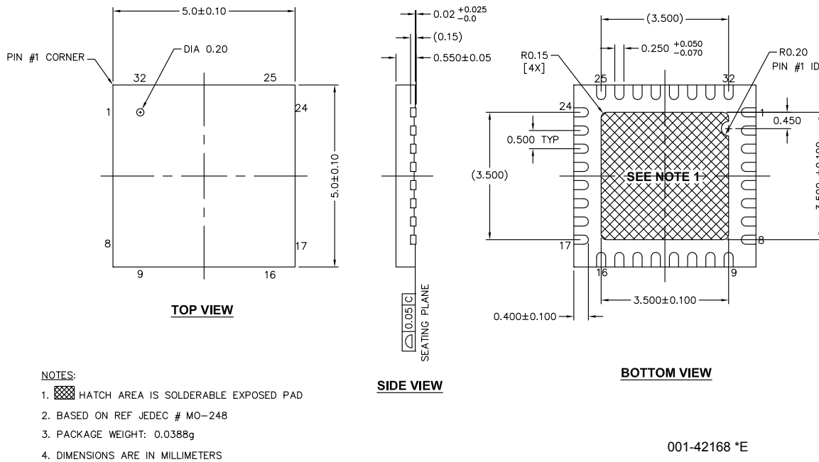
Figure 22. 32-pin QFN (5 × 5 × 0.55 mm) LQ32 3.5 × 3.5 E-Pad (Sawn) Package Outline, 001-42168
