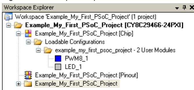
Figure 4-9. Workspace Explorer
