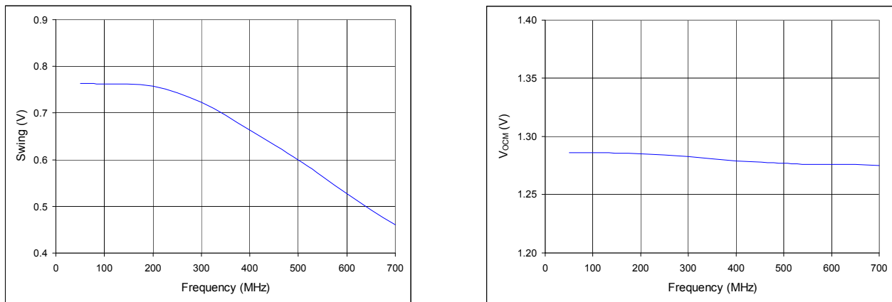
Figure 9. 2.5-V Supply and Termination to V_{DD} -2 V, minimum V_{DD} and maximum T_A
