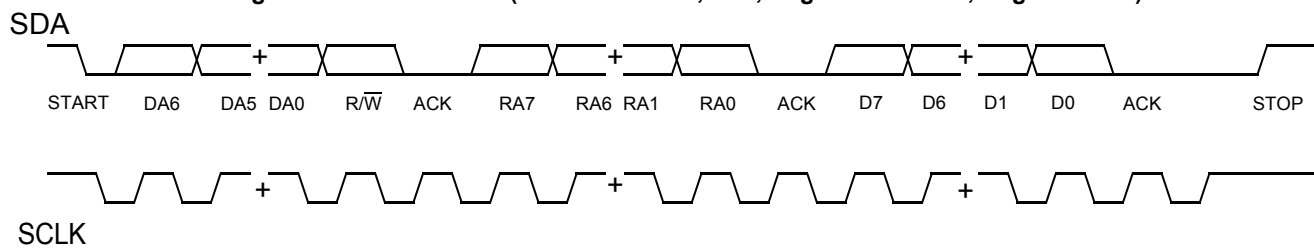
Figure 7. Frame Format (Device Address, \overline{R/\overline{W}} , Register Address, Register Data)
