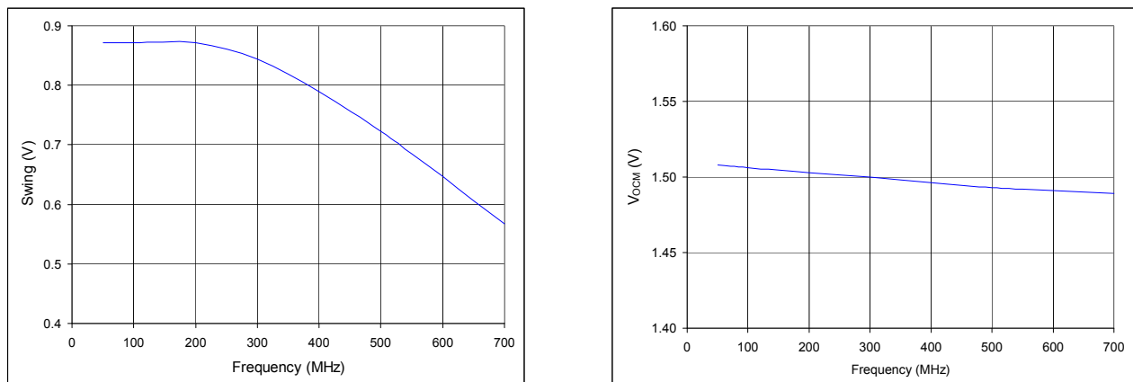
Figure 10. 3.3-V Supply and Termination to V_{DD} -2 V, minimum V_{DD} and maximum T_A
