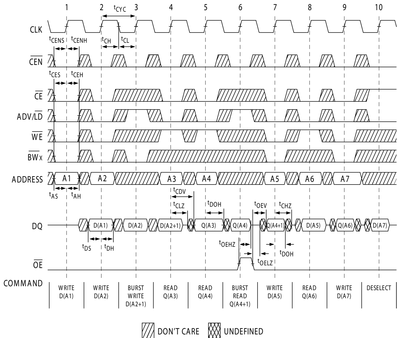
Figure 3. Read/Write Timing [22, 23, 24]
