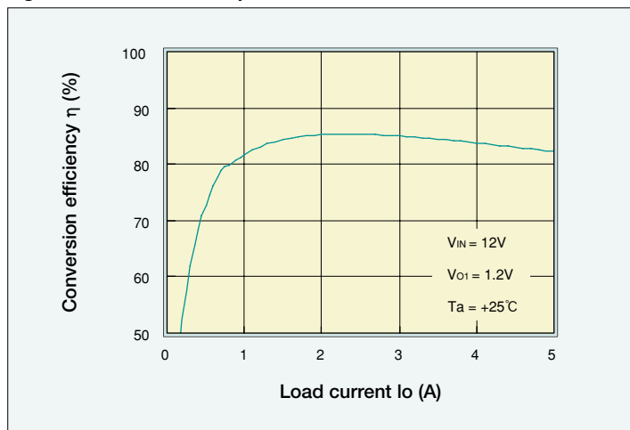
Figure 3 Conversion Efficiency/Load Current (Vo1)
