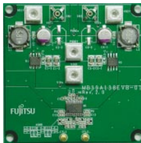
Photo 2 Evaluation Board
