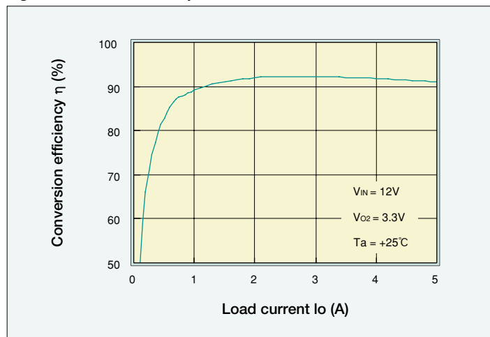
Figure 4 Conversion Efficiency/Load Current (Vo2)
