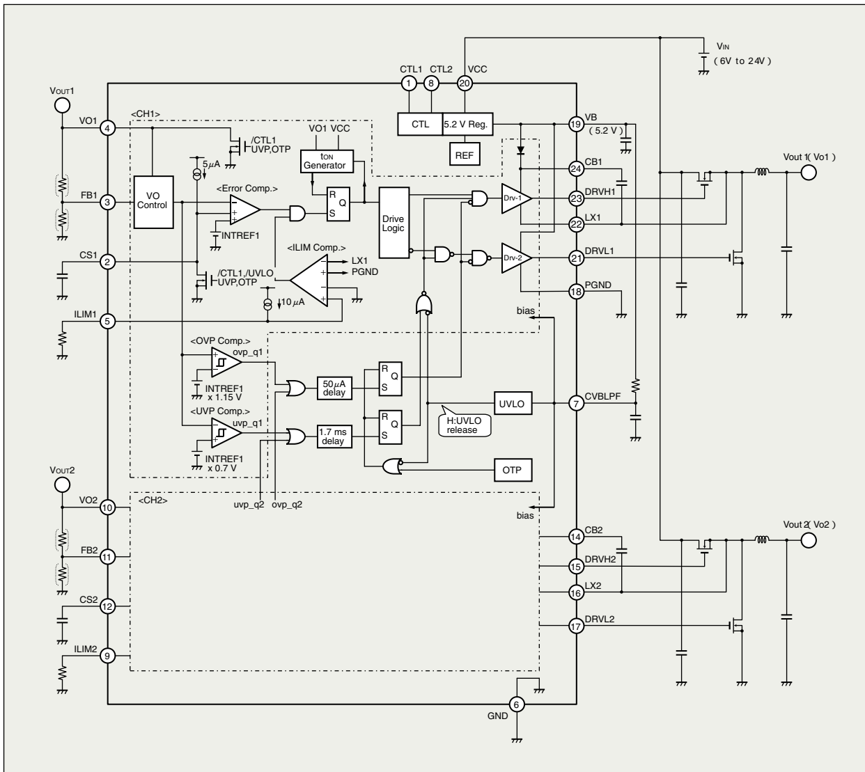
Figure 5 Block Diagram
