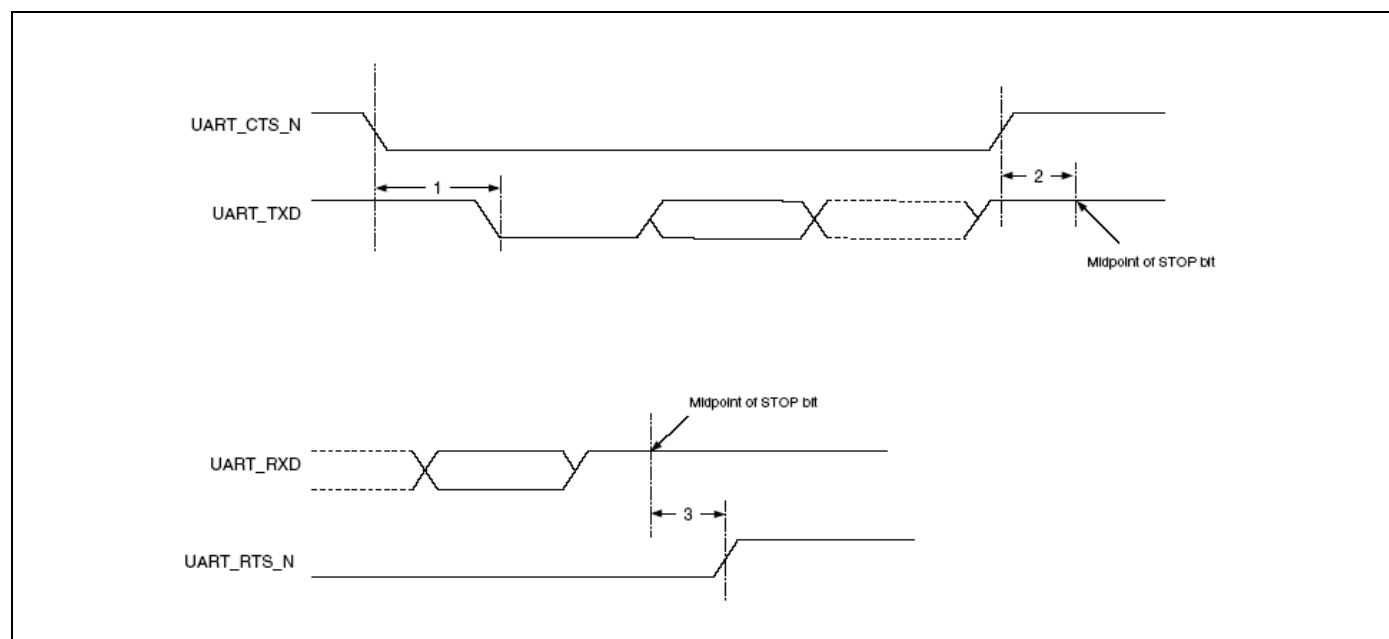
Figure 10. UART Timing
