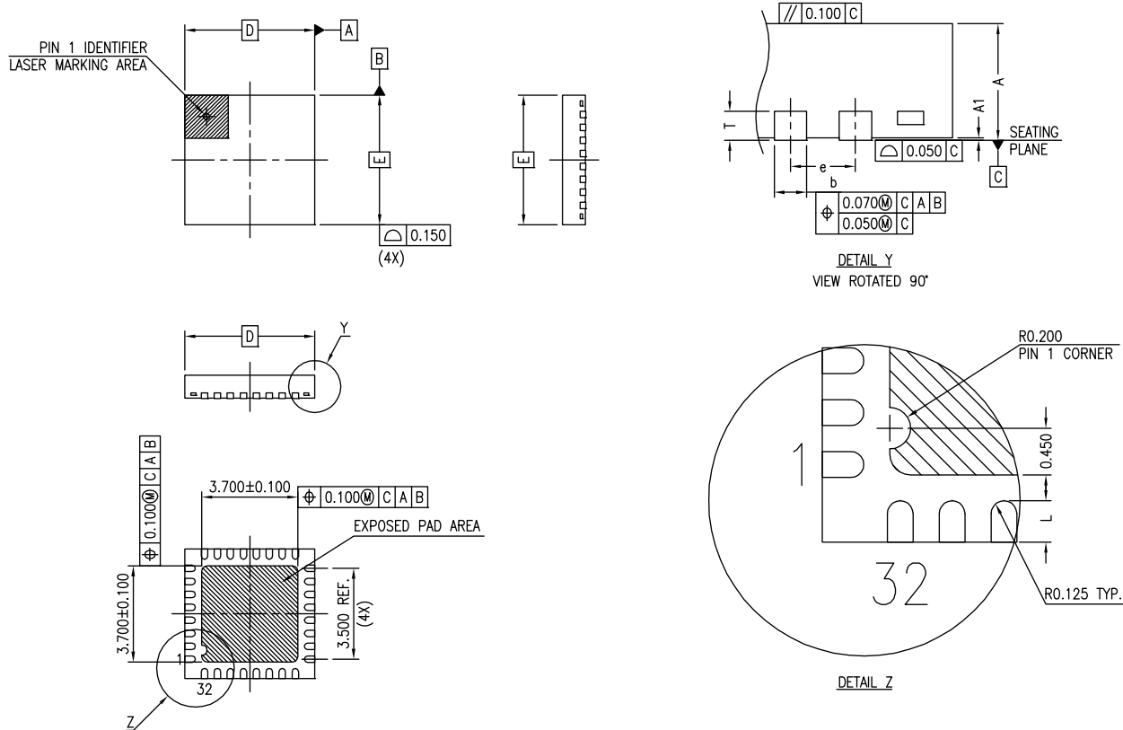
Figure 14. 32-pin QFN
