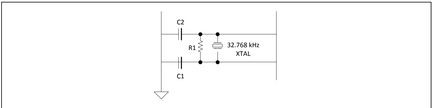
Figure 7. 32 kHz Oscillator Block Diagram
