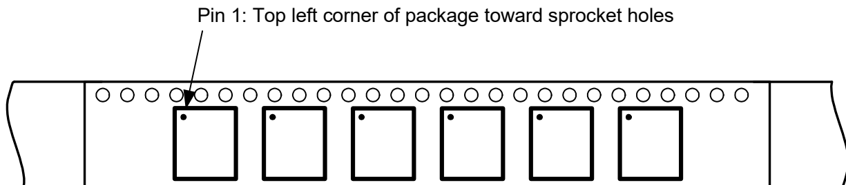
Figure 17. Pin 1 Orientation
