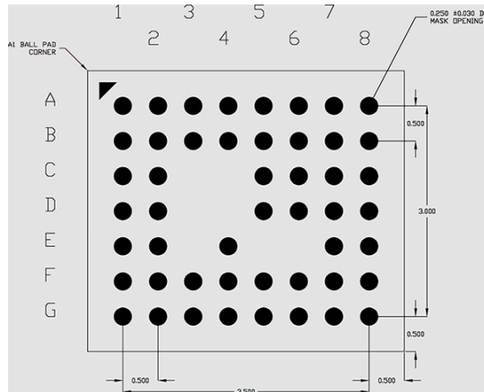
Figure 7. 4.5 mm x 4 mm x 0.8 mm (FcBGA) Array
