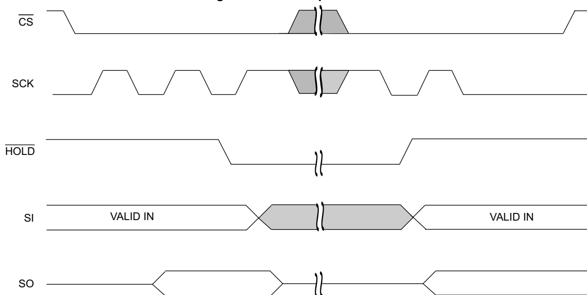
Figure 12. \overline{\text{HOLD}} Operation [2]
