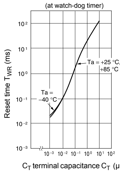
Reset time vs. C_T terminal capacitance (at watch-dog timer)
