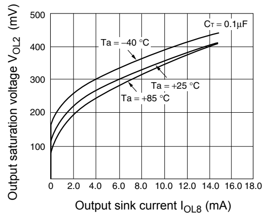
Output saturation voltage vs. Output sink current (RESET terminal)
