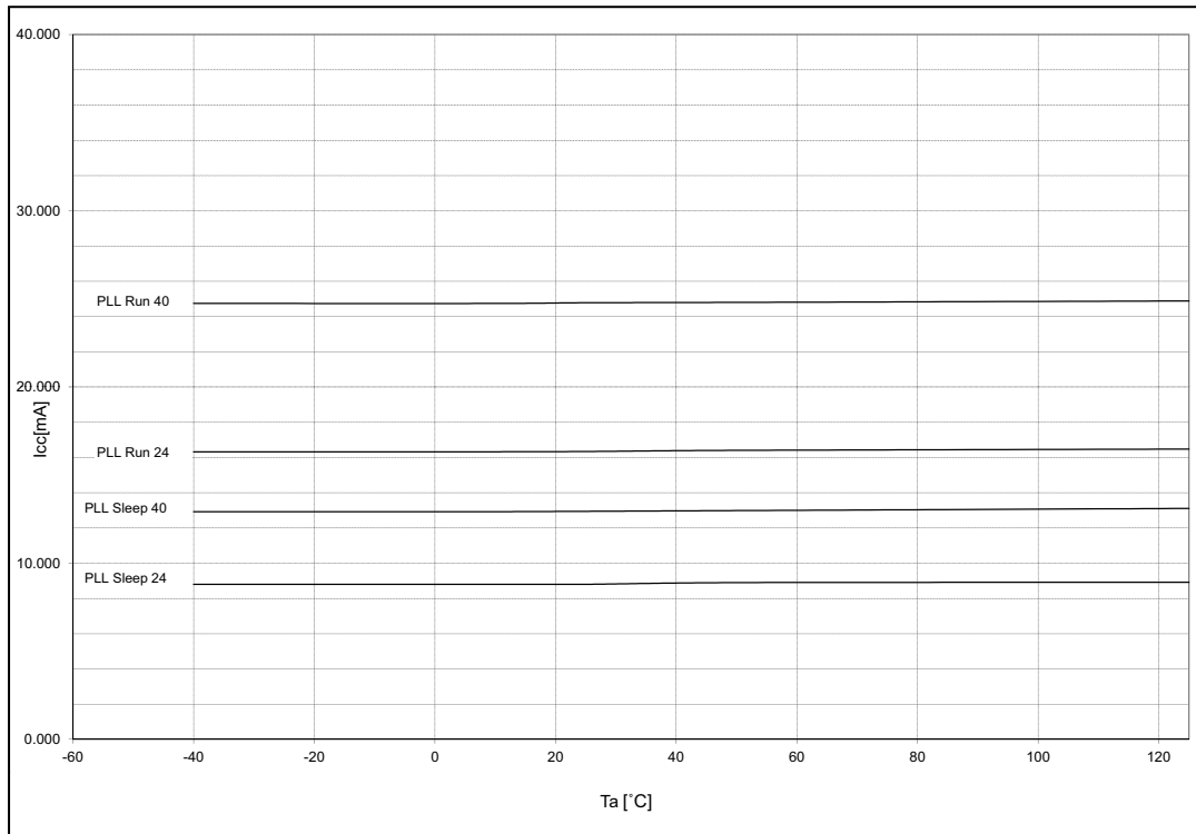
MB96375 PLL Run and Sleep mode currents
