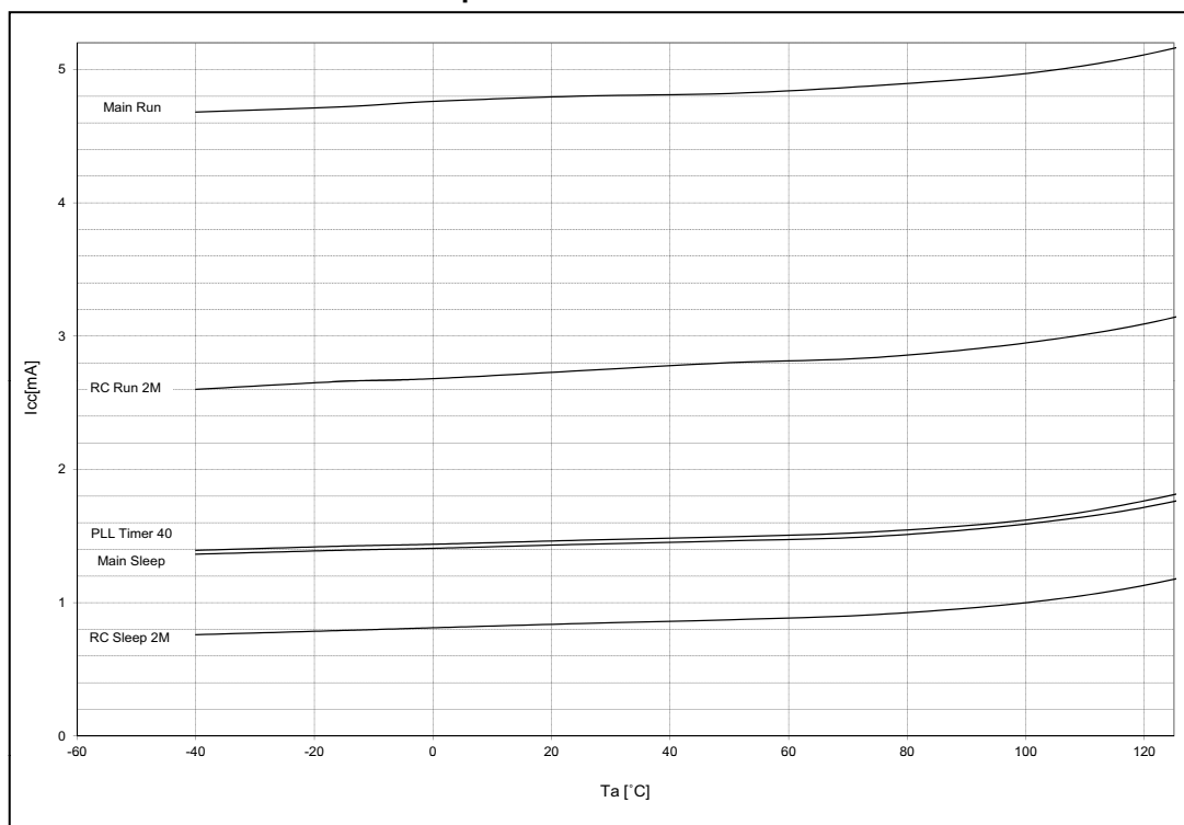
MB96F378/F379 operation modes with medium currents
