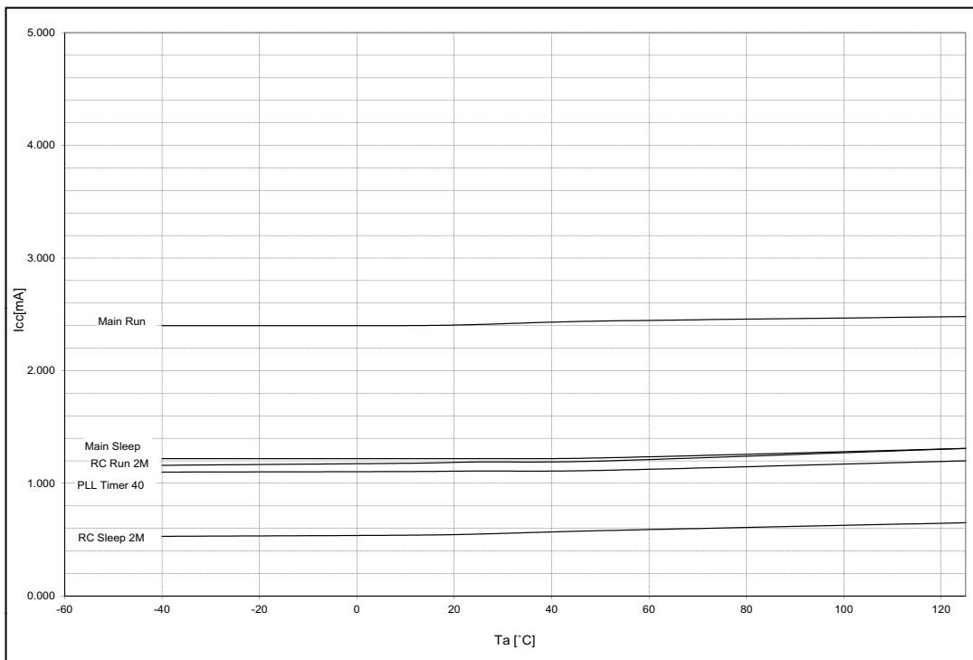
MB96375 operation modes with medium currents
