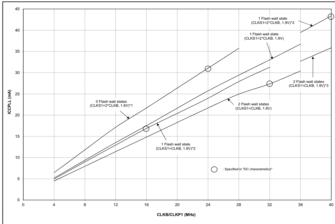
MB96F378/F379 PLL Run mode currents
