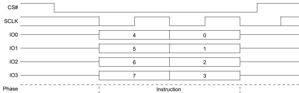
Figure 103. DPD Command Sequence QPI Mode
