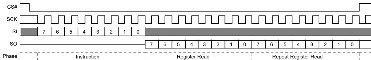
Figure 9.2 PPB Lock Register Read Command Sequence
