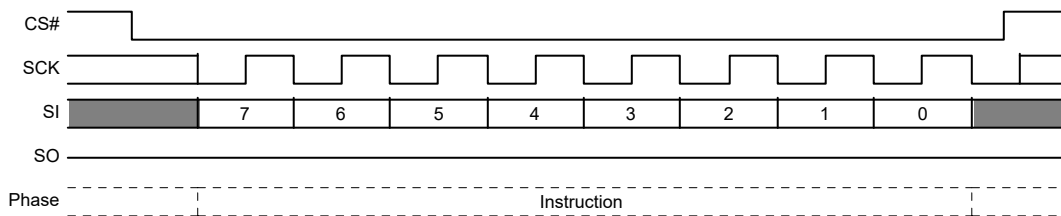
Figure 98. Software Reset Command Sequence
