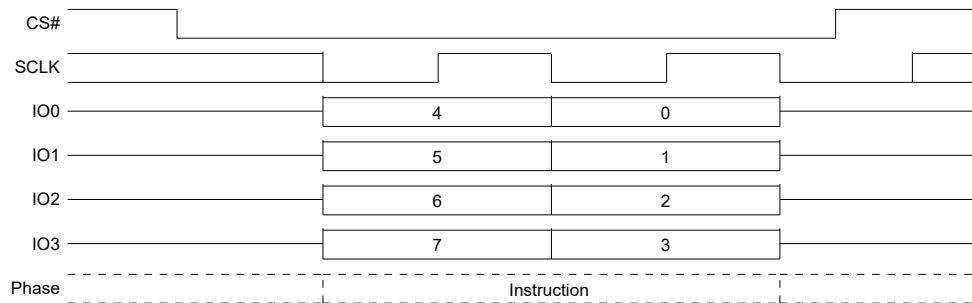
Figure 105. RES Command Sequence QPI Mode
