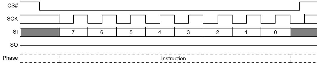
Figure 100. Mode Bit Reset Command Sequence
