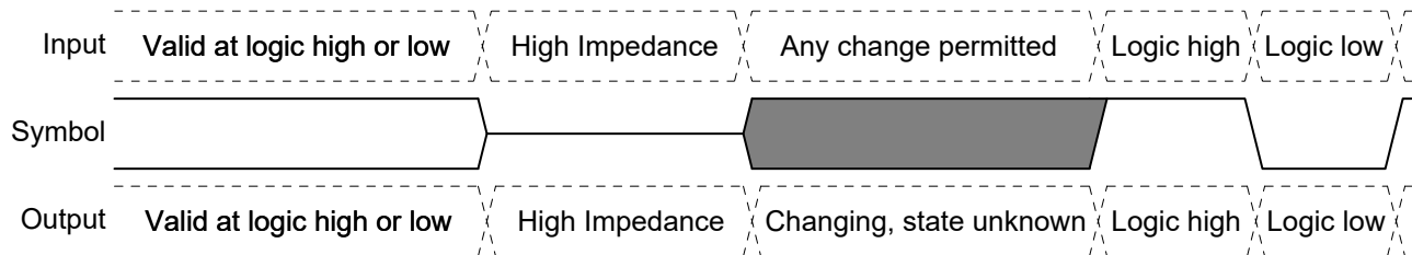
Figure 20. Waveform Element Meanings
