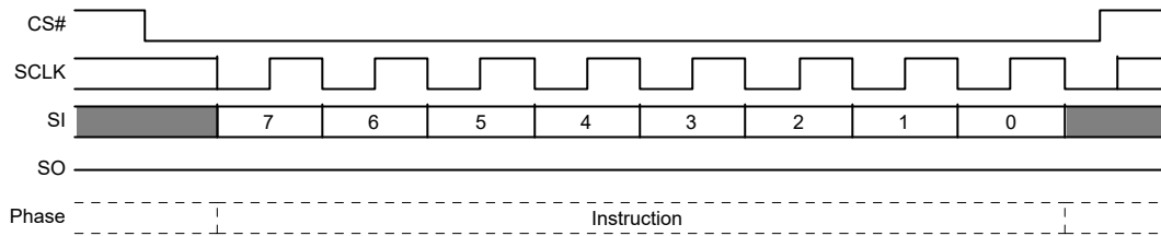
Figure 104. Release from Deep Power-down Command Sequence
