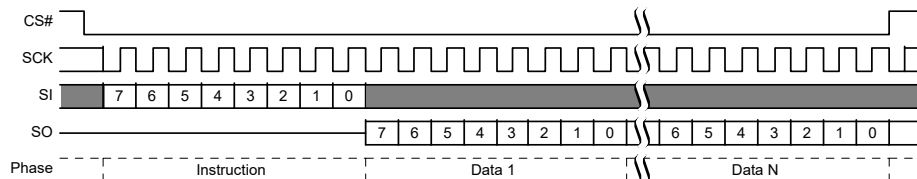
Figure 96. Password Read Command Sequence
