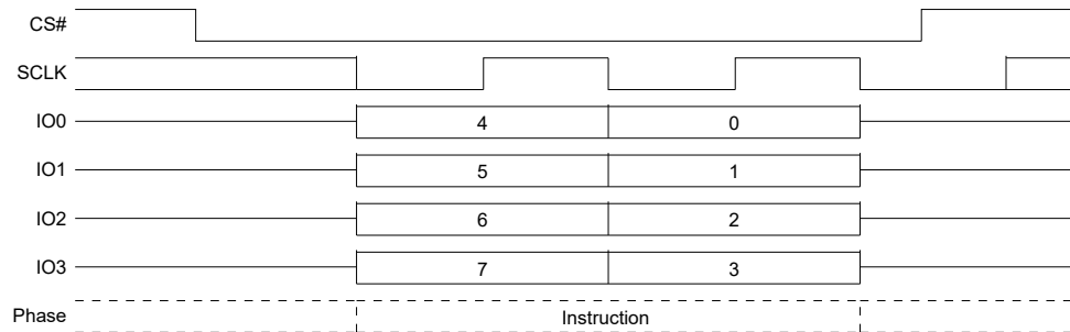
Figure 101. Mode Bit Reset Command Sequence QPI Mode
