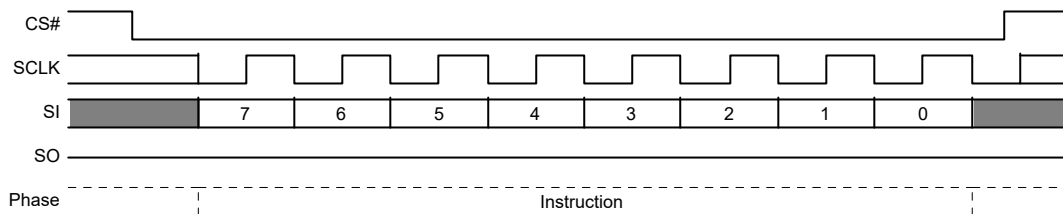
Figure 102. Deep Power-down Command Sequence
