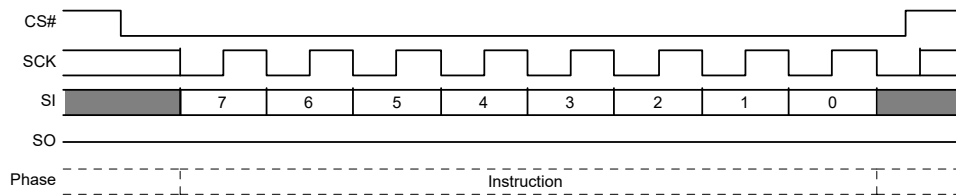
Figure 95. PPB Lock Bit Write Command Sequence
