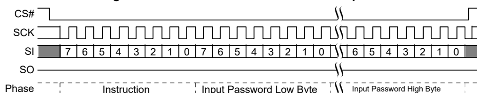
Figure 97. Password Unlock Command Sequence
