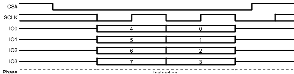
Figure 99. Software Reset Command Sequence QPI Mode
