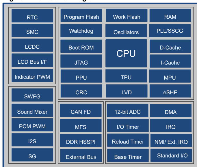
Figure 1: Functional Diagram
