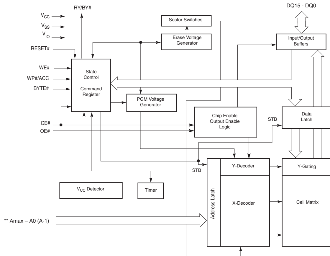
Figure 1.1 Block Diagram
