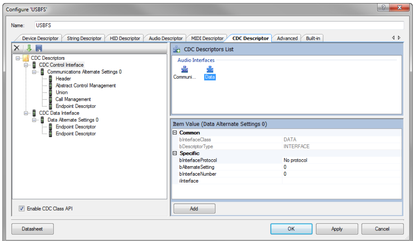
Figure 5-60. USBFS Component CDC Descriptor Configuration
