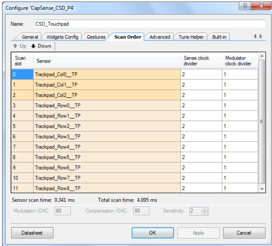
Figure 5-20. Scan Order Tab of CapSense Gesture Component
