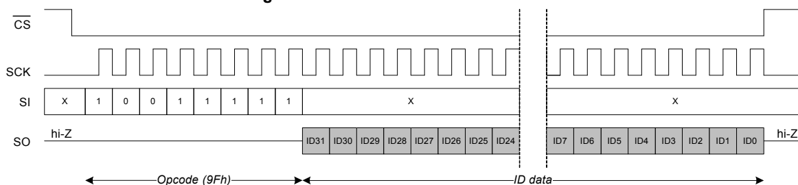
Figure 73. RDID Instruction in SPI Mode
