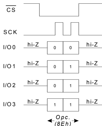
Figure 96. ASEN Instruction in QPI Mode
