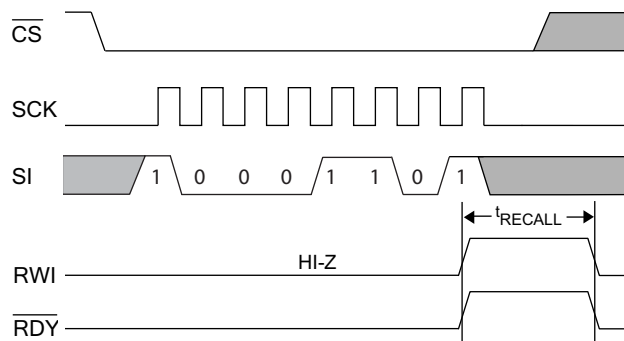
Figure 108. Software RECALL Cycle [22]
