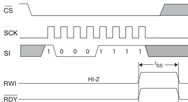
Figure 110. AutoStore Disable Cycle
