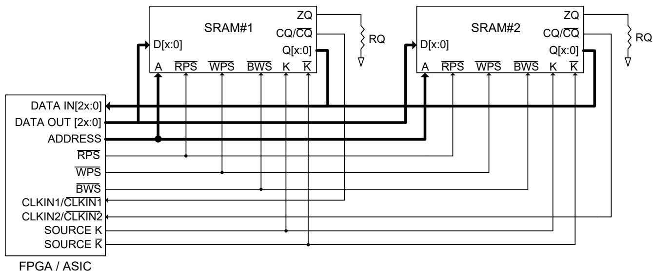
Figure 2. Application Example
