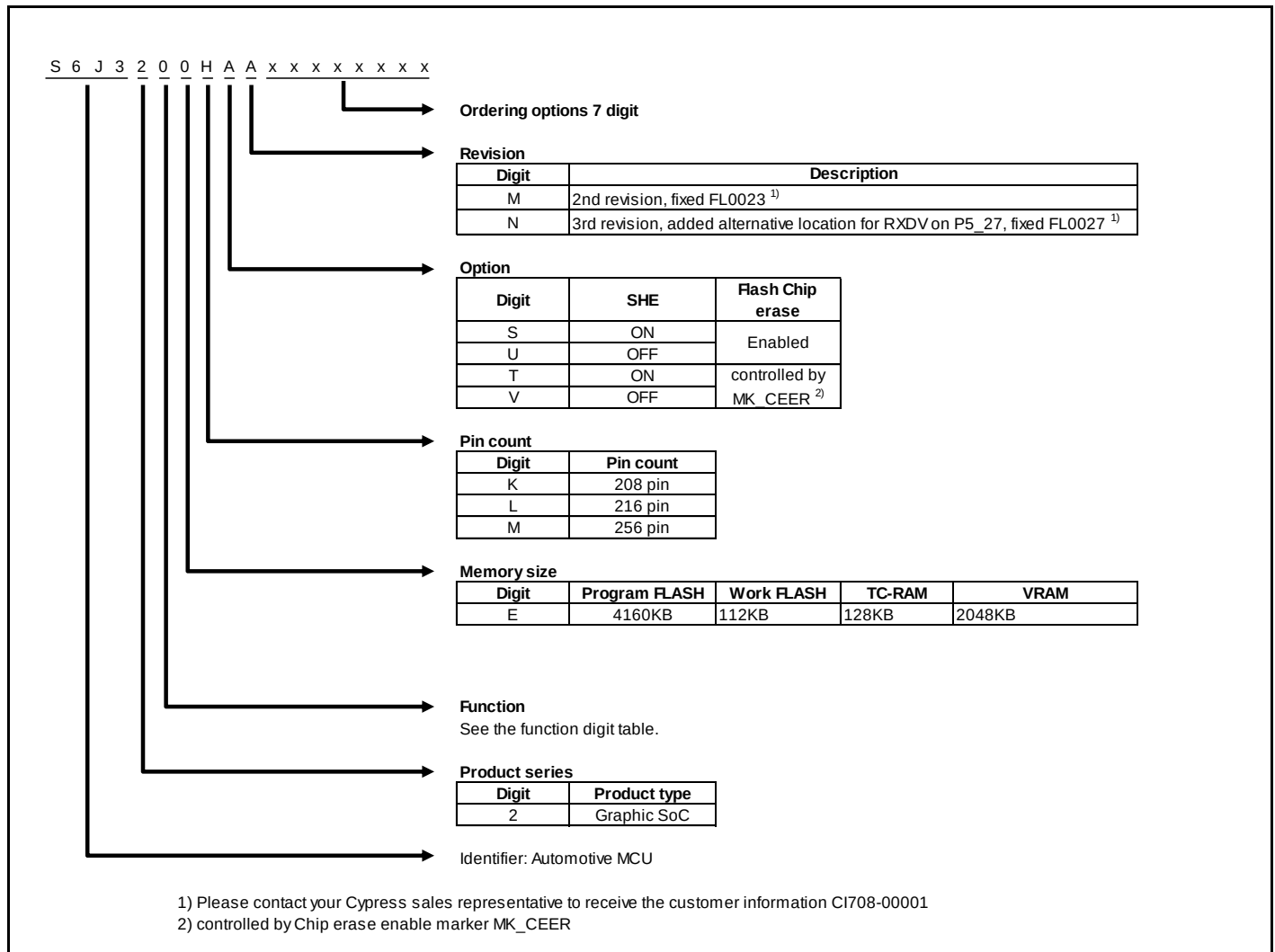
Figure 2-1: Option and Part Number
