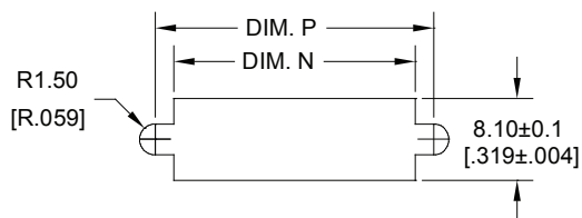
Panel Thickness: 2.0 mm (.08 inch) Max.
