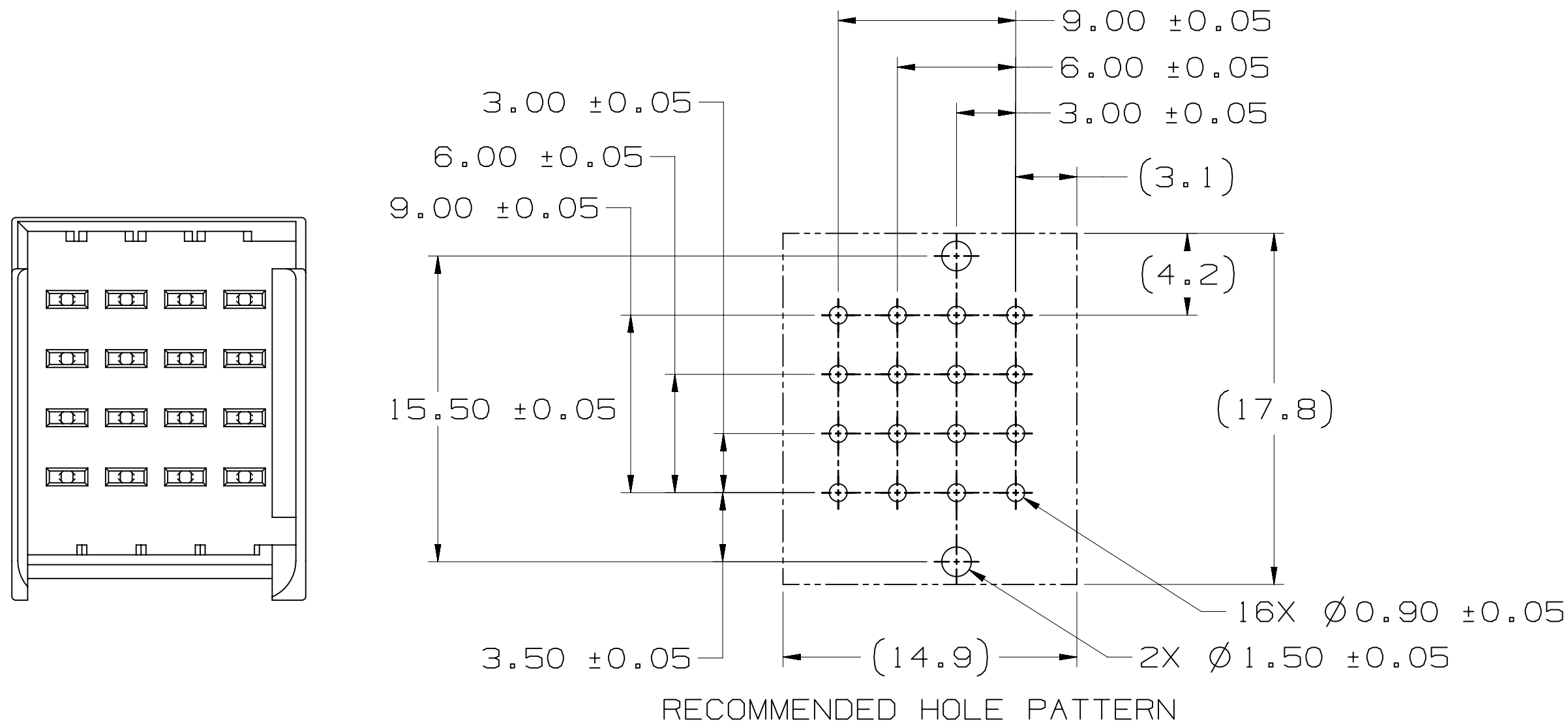
16 POSITION 3S616-62X4-B00 PP
