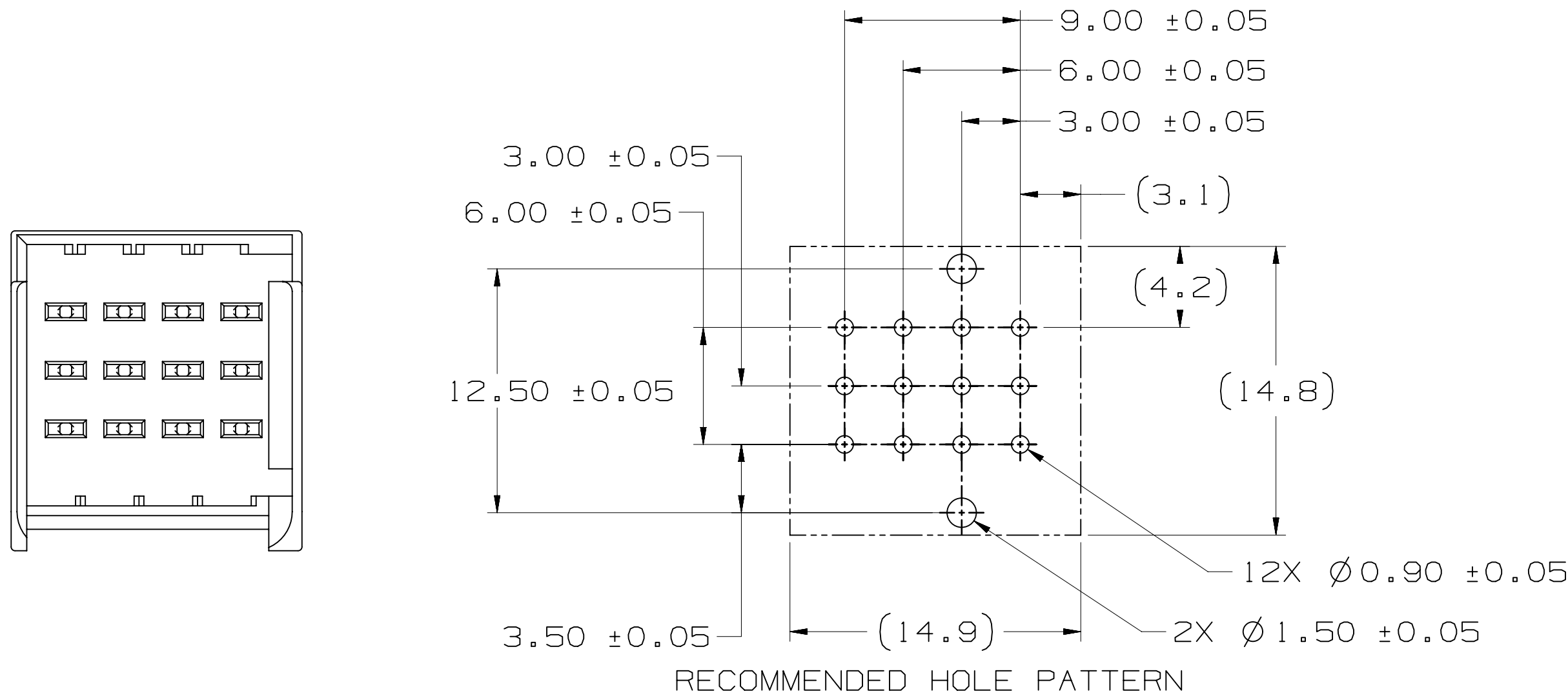
12 POSITION 3S612-62X3-B00 PP
