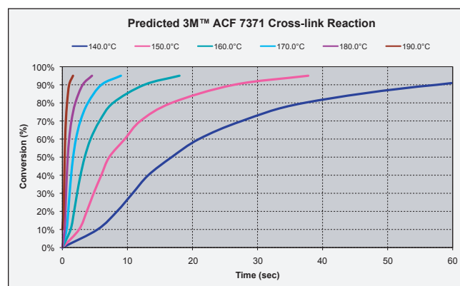
Figure 2. Graph of predicted cross-link reaction compared with bonding temperature and time.
