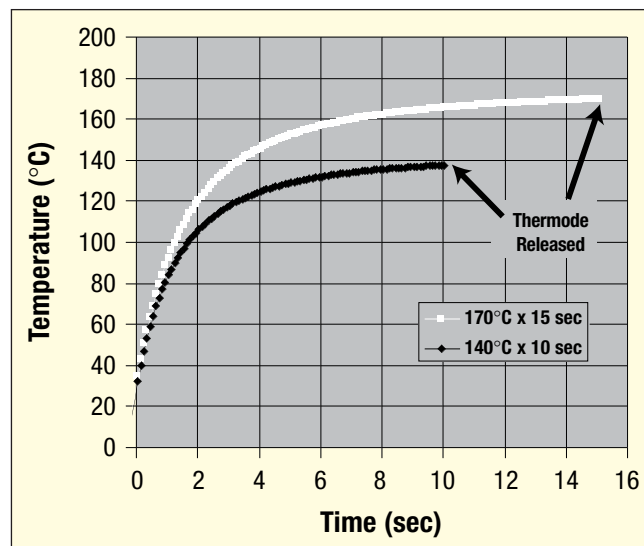
Figure 1. Graph of ACF temperature vs. time profile showing typical examples of bonding cycle.
