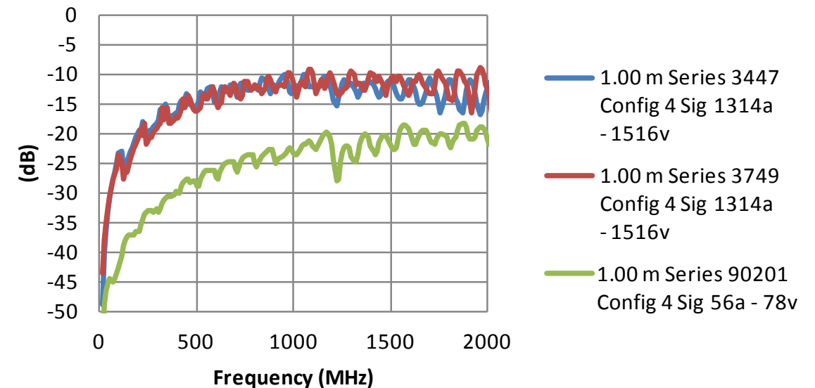
1.0 m (39.4 in.) Diff. FEXT
