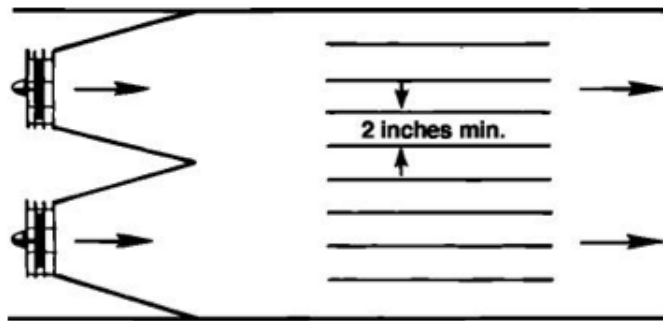
Figure 1: Schematic Drying Set-up for Air Drying
