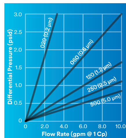
Graph 2: Clean Water Flow per 10" Betafine™ PBG Series Filter Cartridge at Ambient Temperature (20°C)
