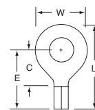
MU14-14RHT Stud Size 1/4 Wire Range 16-14
