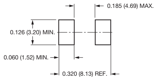
Mounting Pad Layout
