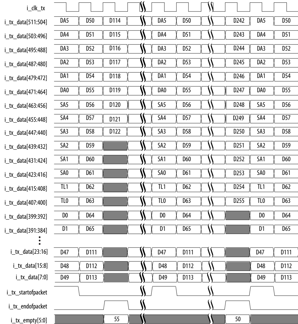
The figure illustrates how the octets of the client frame are transferred over the TX datapath when preamble pass-through is turned off.
