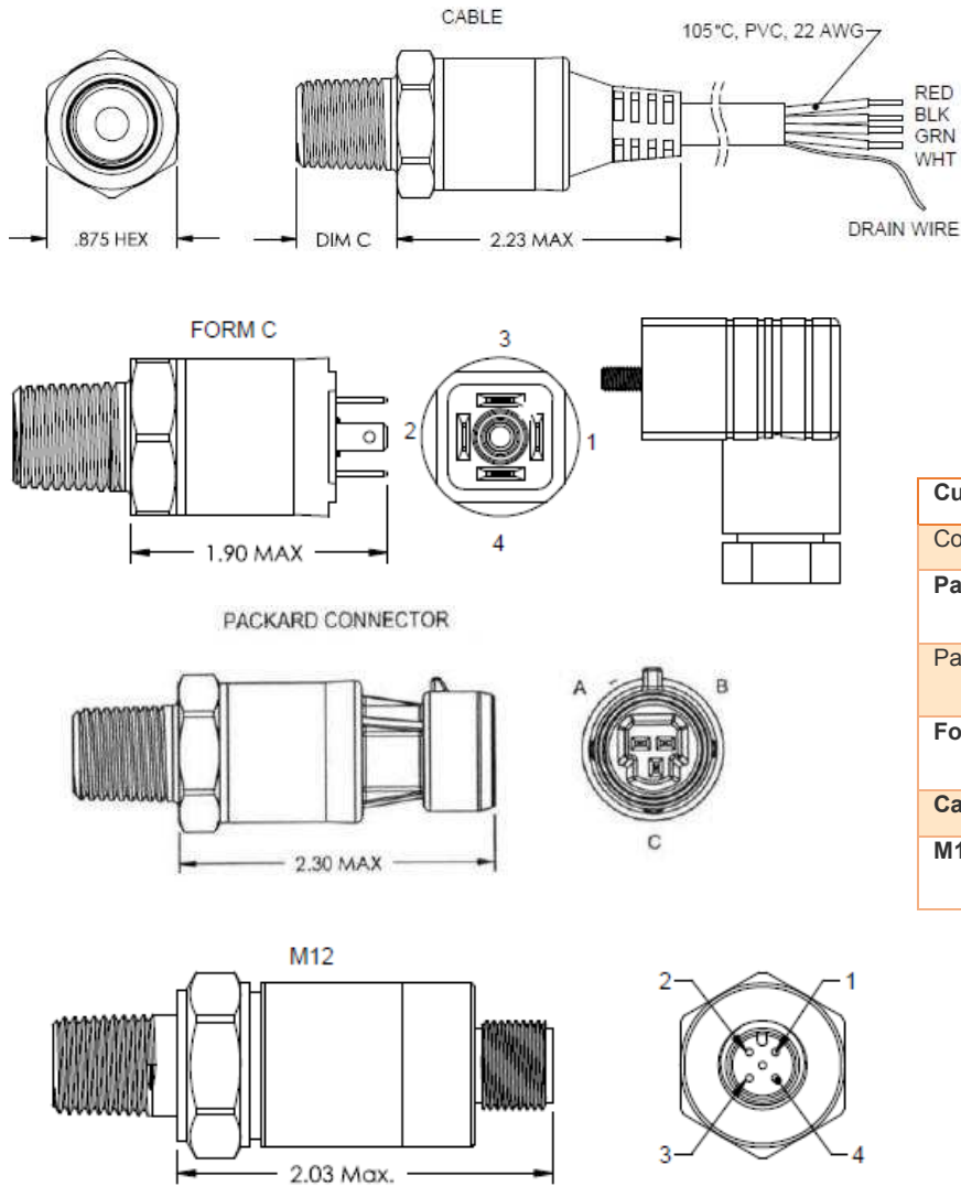
Voltage Output Wiring
