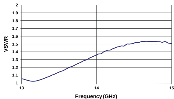
VSWR (13-15 GHz)
