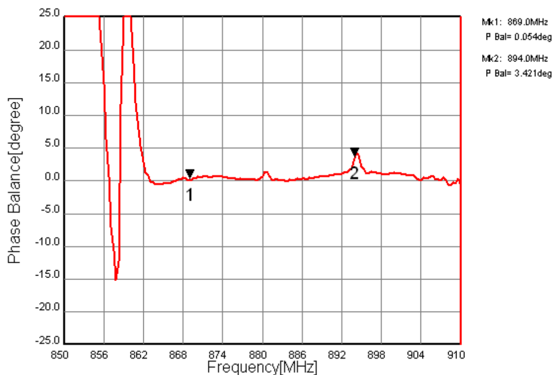
Fig.8 Phase Balance
