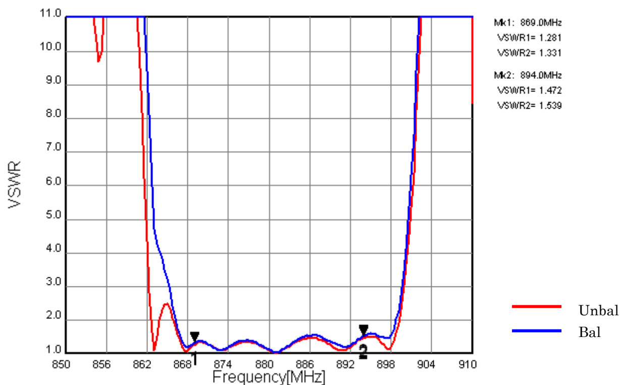
Fig.2 VSWR
