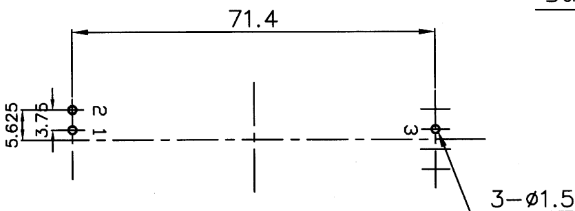
P.C.B. Mounting hole detail
