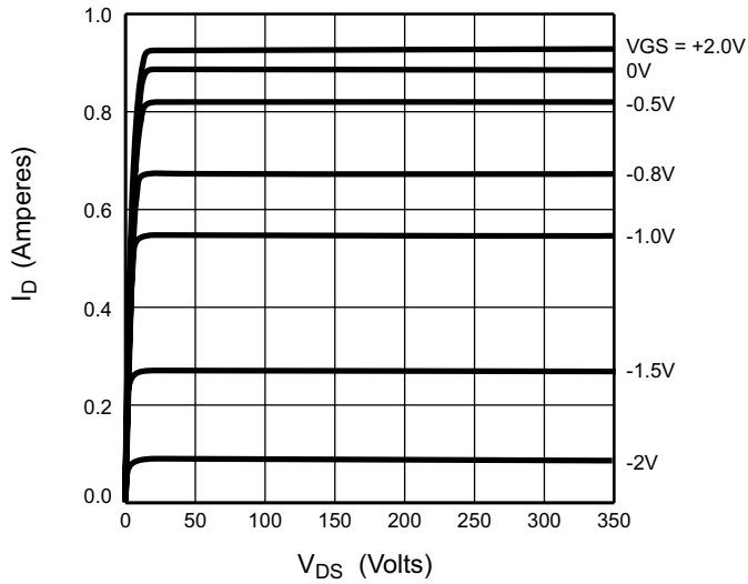
Output Characteristics
