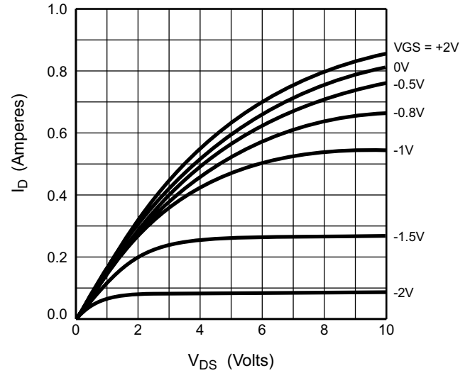
Saturation Characteristics
