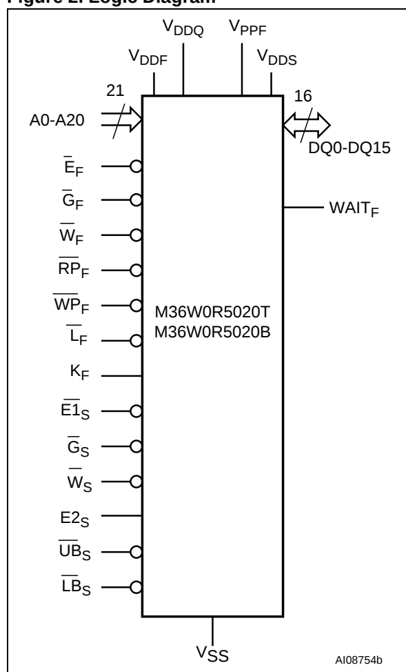
Figure 2. Logic Diagram
