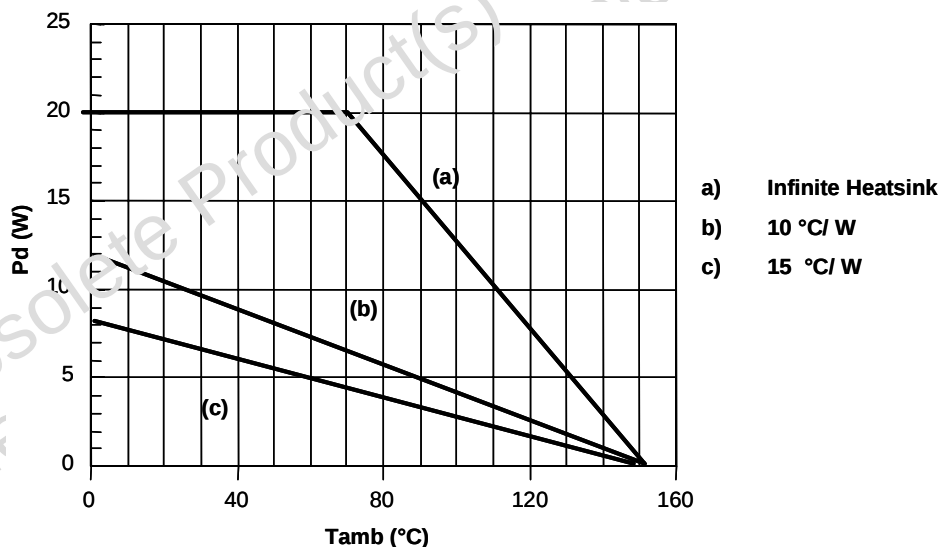
Figure 10. Power Derating Curve
