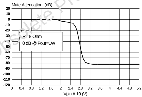
Mute Attenuation vs. Vpin 10
