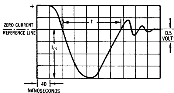
TYPICAL OSCILLOSCOPE PATTERNS OF RECOVERY
