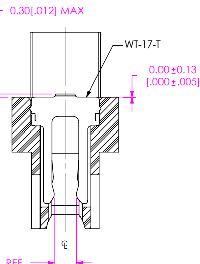
SECTION "B"- "B" SCALE 4 : 1
