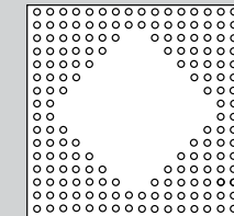
-16=172 Pins
