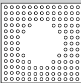
-13B=132 Pins
