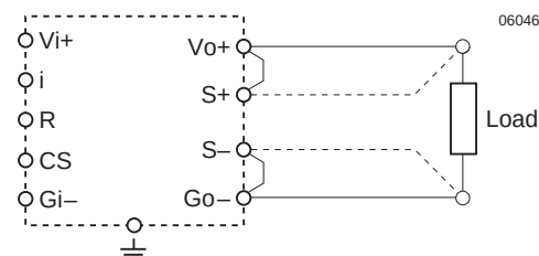
Fig. 5 Sense lines connection
