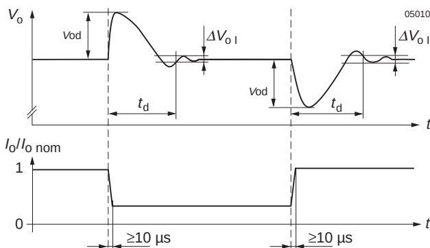
Fig. 2 Dynamic load regulation.
