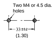
Mounting holes
