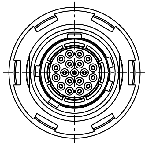
GKAYC R-P19W CDO-000L Mechanical coding: C Color coding: blue
