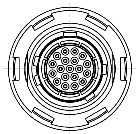
GKAYBR-P19WCD0-000L Mechanical coding: B Color coding: red
