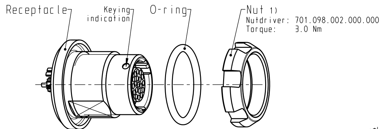
GKAYAR-P19WCD0-000L Mechanical coding: A Color coding: light brown
