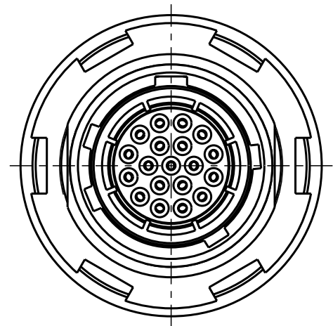
GKAYDR-P19WCD0-000L Mechanical coding: D Color coding: green
