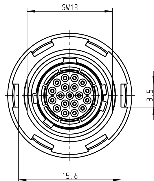
GKAYAR-P19WCD0-000L Mechanical coding: A Color coding: light brown
