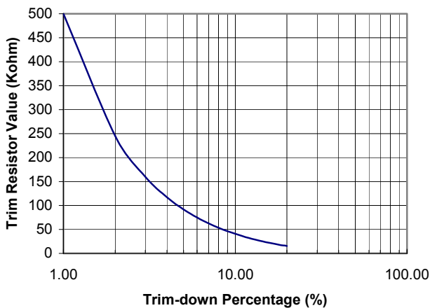
Figure 12. Trim-Down Resistor Selection
