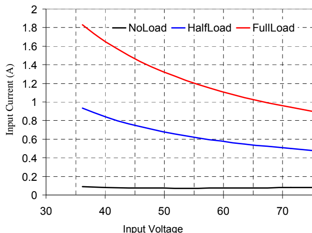
Figure 2. Input Characteristics
