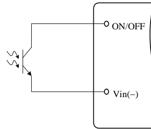
Figure 9. Opto Coupler Enable Circuit
