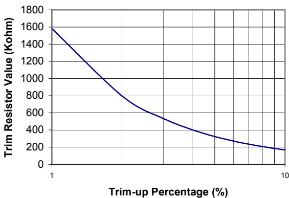
Figure 13. Trim-Up Resistor Selection
