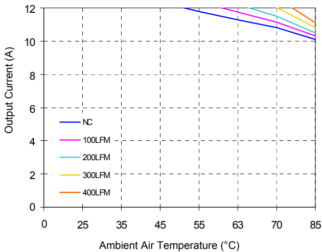
Figure 7. Current Derating Curve for Airflow Direction 1 (Ref. Figure. 8 for Airflow Direction; typical Vin, open frame, unit soldered onto a fixture board.)
