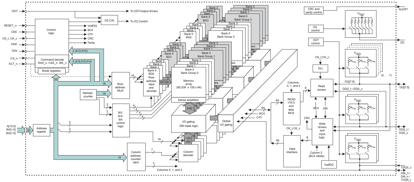
Figure 2: 1 Gig × 8 Functional Block Diagram
