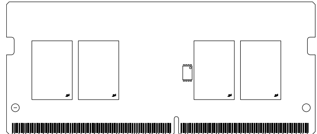
Figure 1: 260-Pin SODIMM (MO-310 R/C A1, R/C A2)
