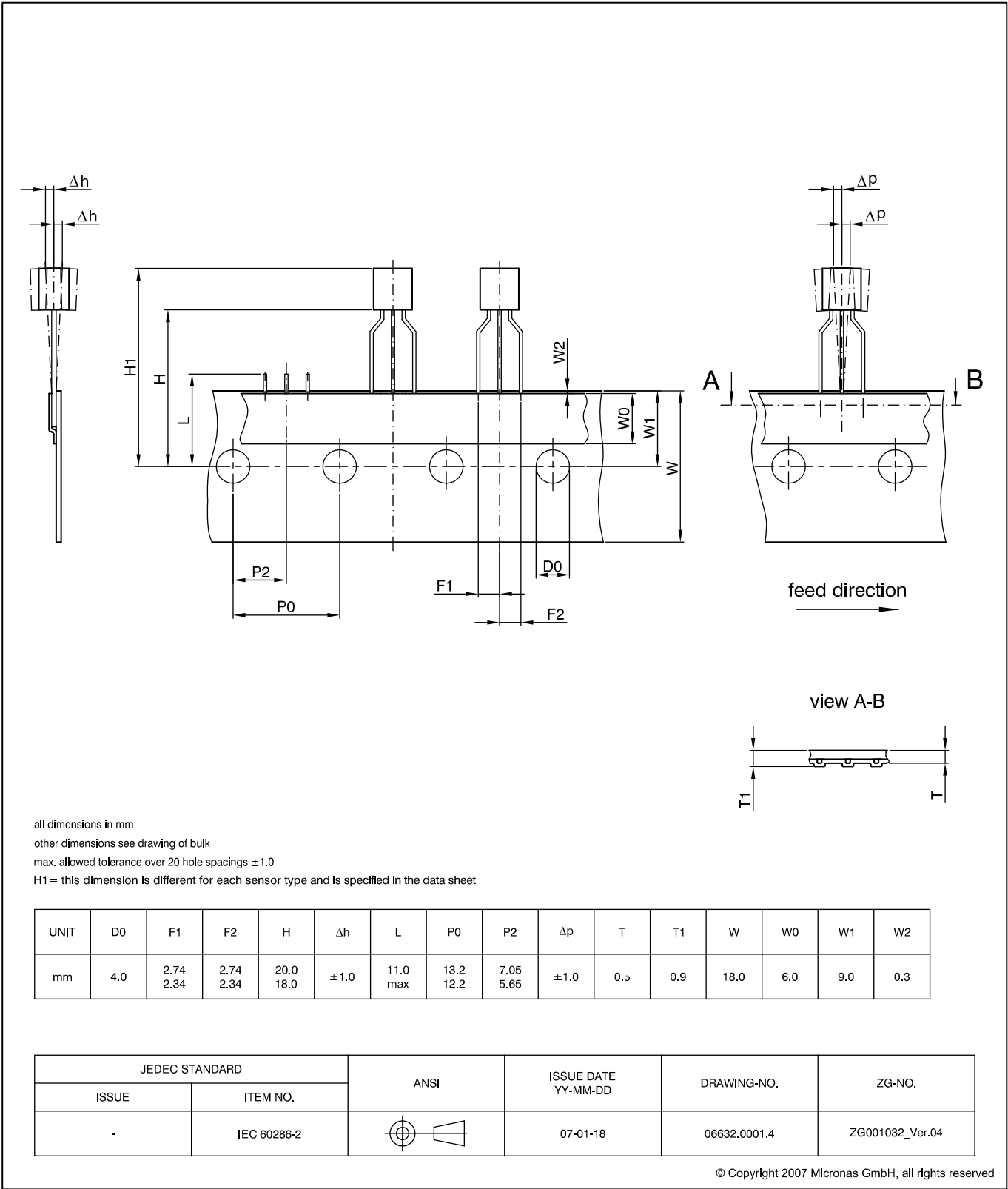
Fig. 4–4: TO92UA/UT: Dimensions ammopack inline, spread
