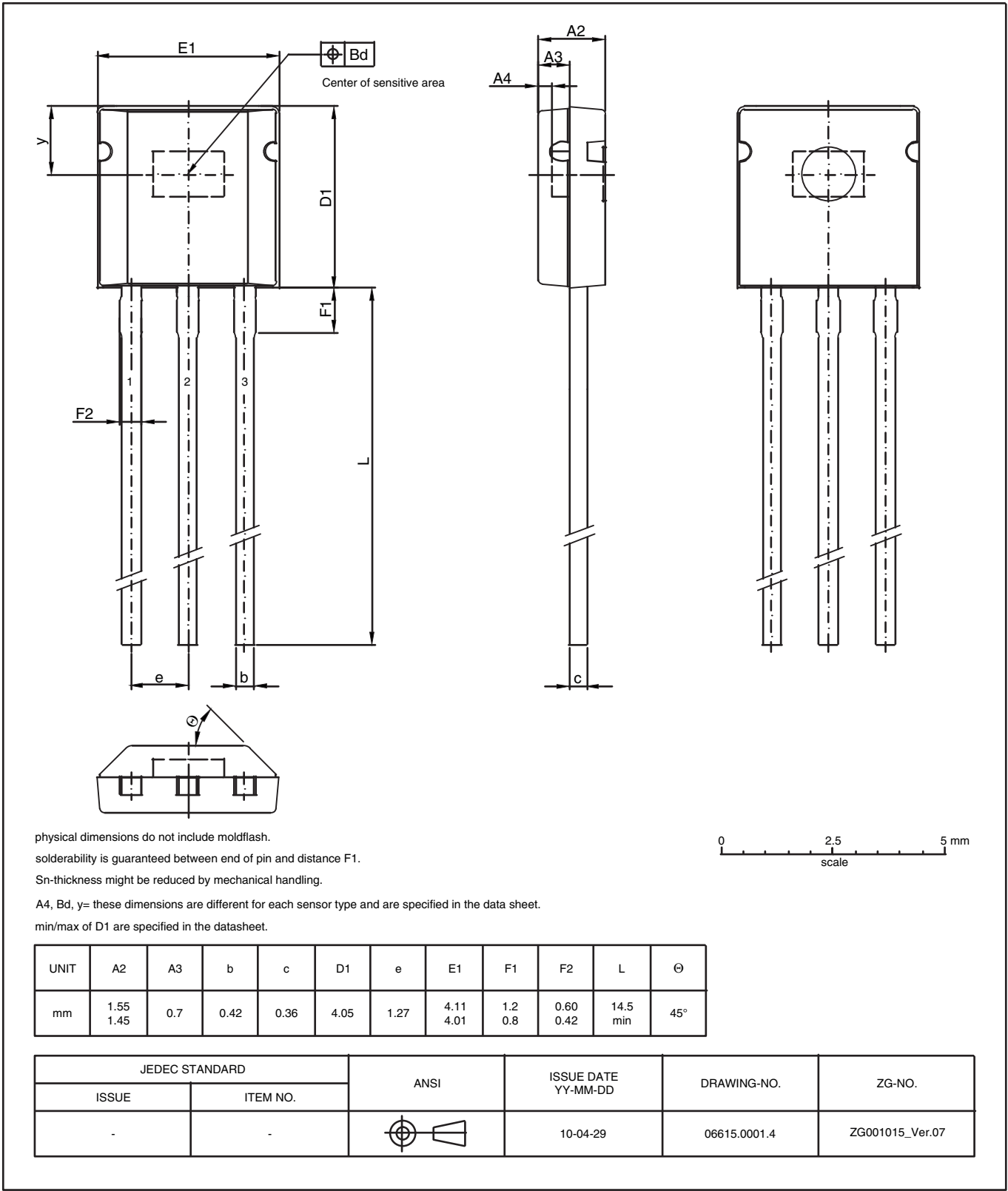
Fig. 4-2: TO92UT-2 Plastic Transistor Standard UT package, 3 leads Weight approximately 0.12 g
