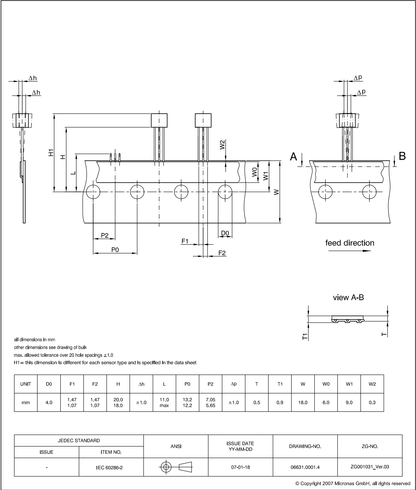
Fig. 4-3: TO92UA/UT: Dimensions ammpack inline, not spread
