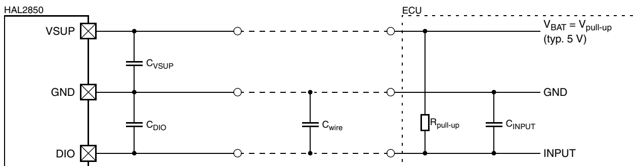
Fig. 7–2: Application circuit for 5 V supply
