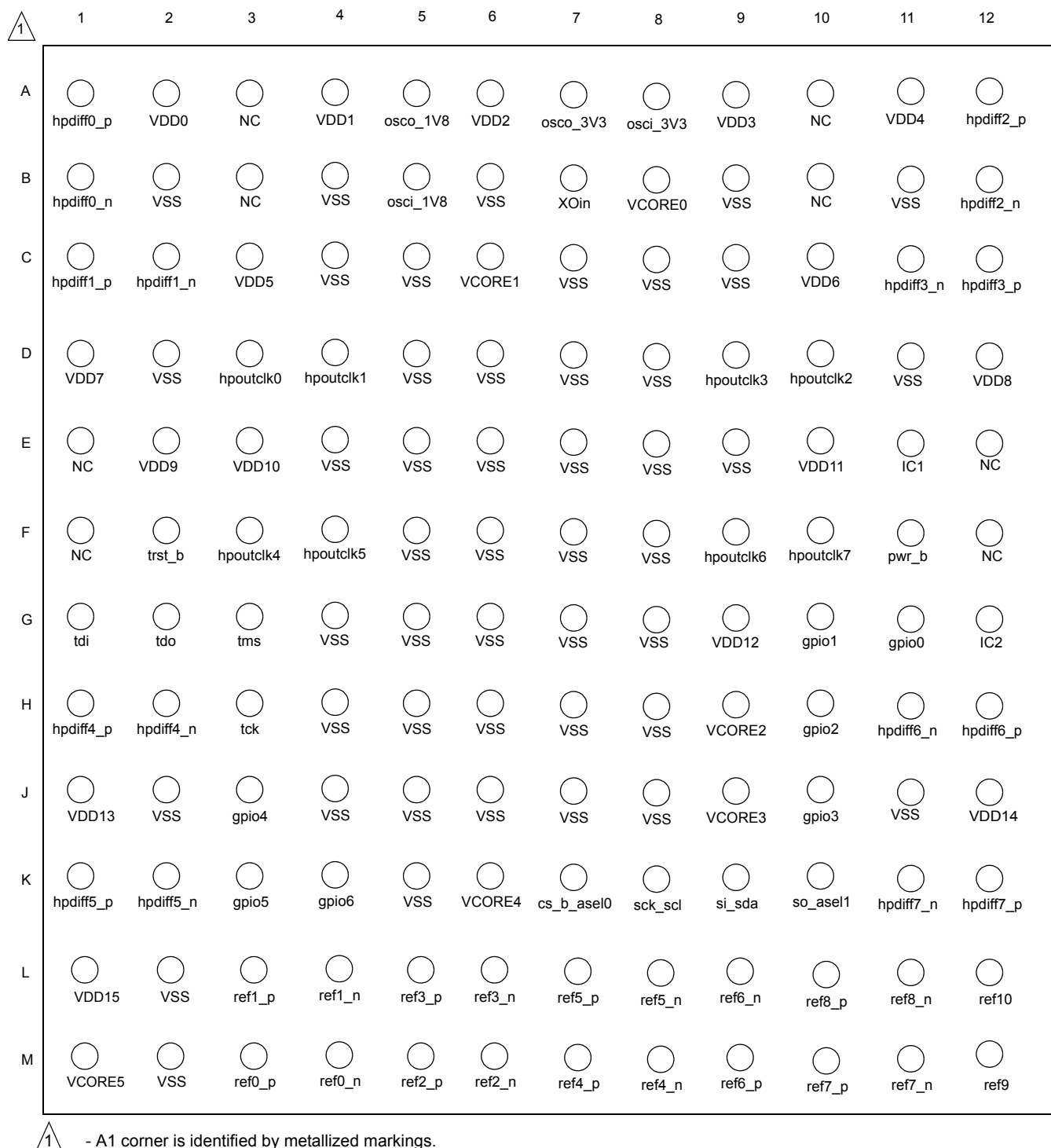
Figure 2 - Package Description
