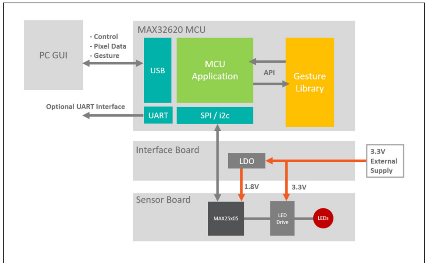
Figure 9. System Diagram
